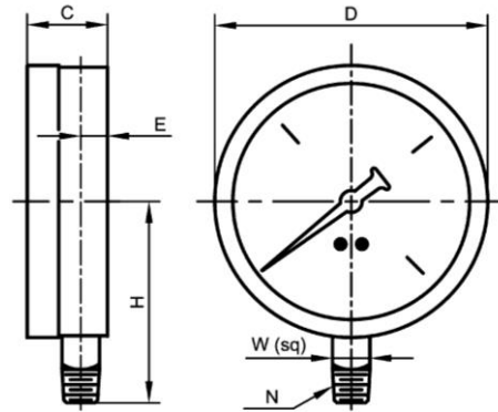
Bottom Connection
